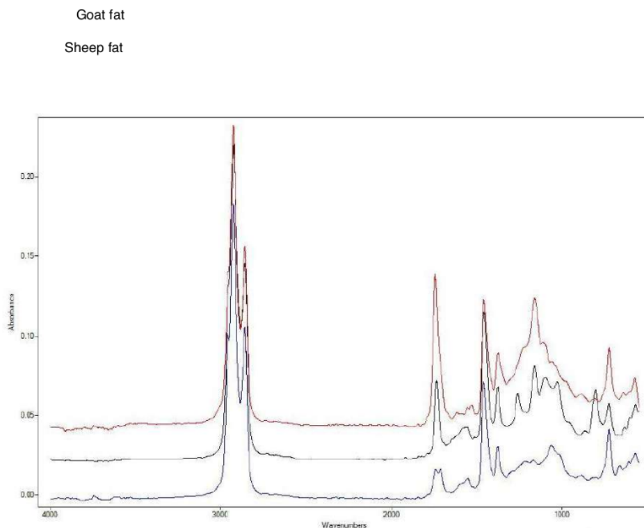
4 Figure 2. FTIR spectra of the lipid extracted from pig, goat, and sheep leather
