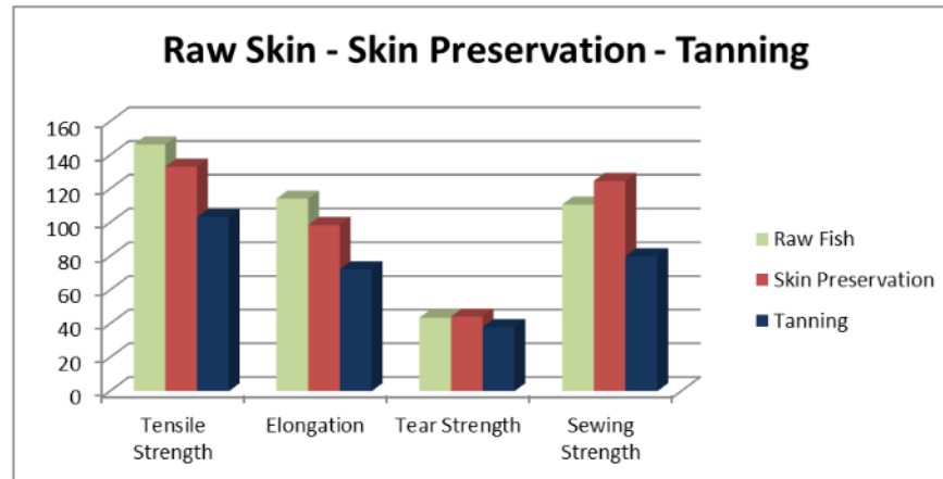
Figure 1. Physical testing results of raw skin, preserved skin and tanned leather
